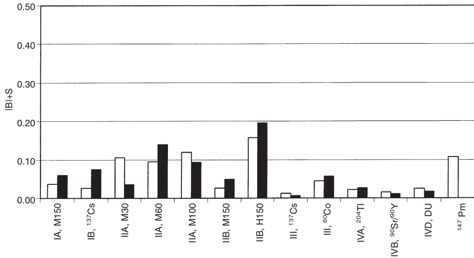
Figure 4. Performance DXT-RAD extremity, |B| + S. □, LiF:Mg,Cu,P; ■, LiF:Mg,Ti.
